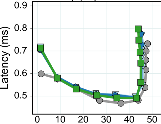
(a) Apache
