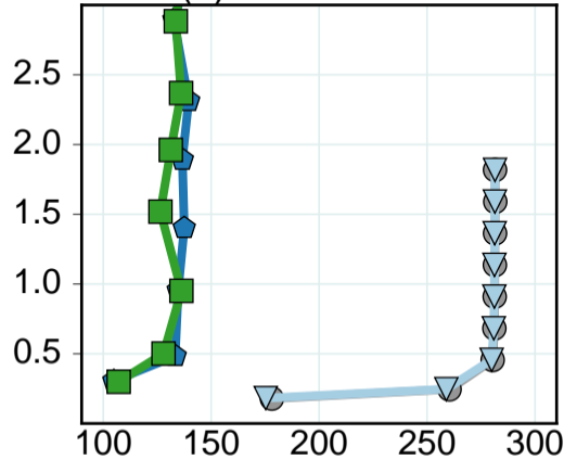
(c) Memcached
