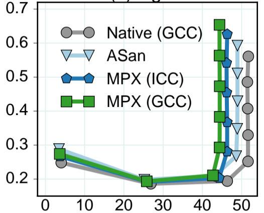
(b) Nginx
