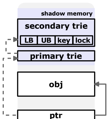
(c) Pointer-based: SoftBound
