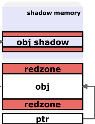
(a) Trip-wire: AddressSanitizer
