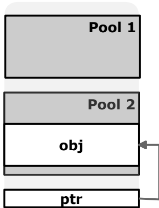
(b) Object-based: SAFECode
